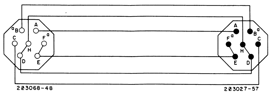
CABLE NO.7
