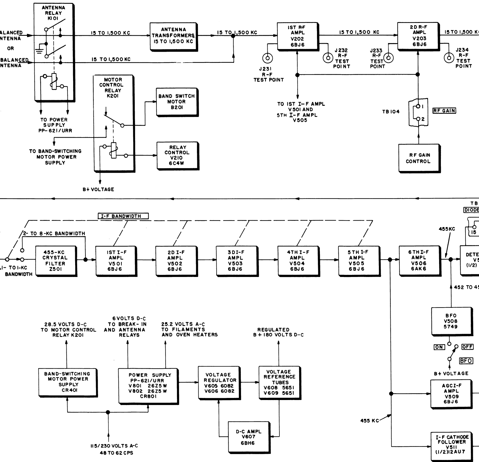
Figure 12. Radio Receiver R-389/URR, block diagram.
