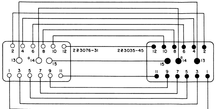
CABLE NO. 6
