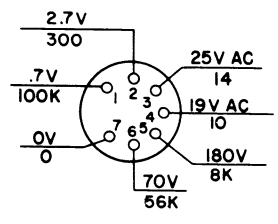
2D MIXER V205 6BE6
