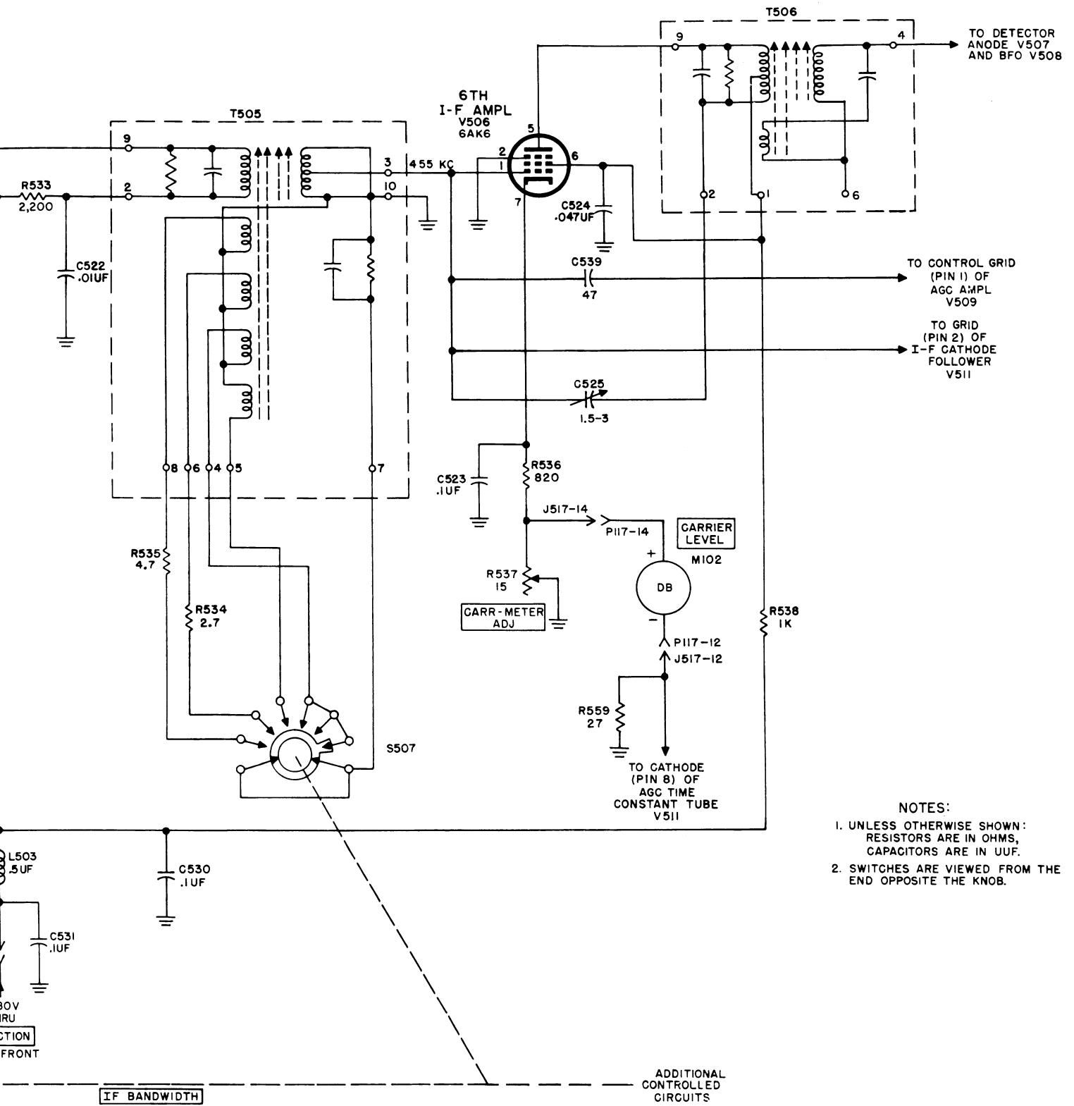
sixth if. amplifiers, schematic diagram.
