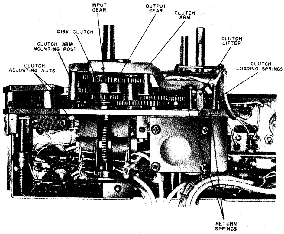
Figure 75. Disk clutch assembly, mounted.
