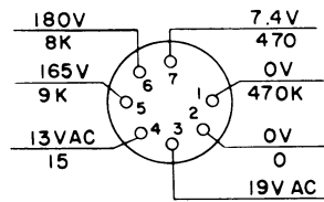
LINE A-F OUTPUT TUBE V604 6AK6
