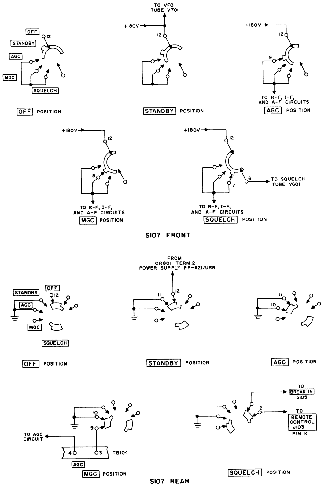
Figure 40. FUNCTION switch, schematic diagram.
