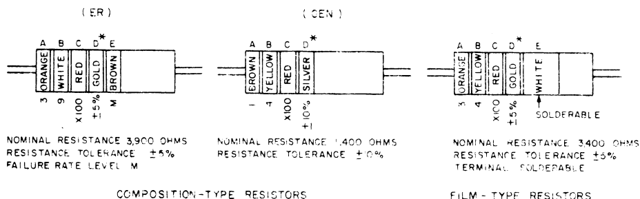
COMPOSITION-TYPE RESISTORS
