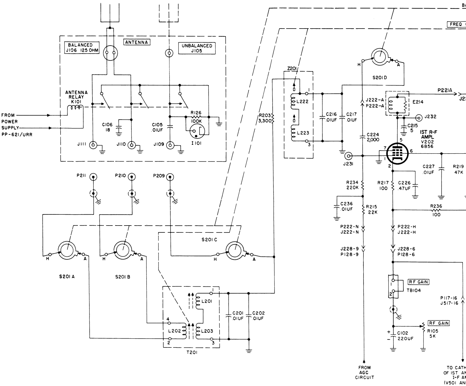
Figure 13. Antenna circuit and first rf amplifier, sheet 1 of 2
