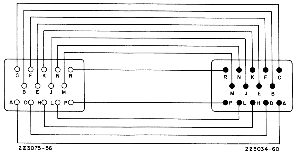
CABLE NO.4
