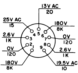
1ST MIXER V204 12AT7
