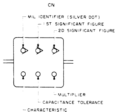
PAPER-DIELECTRIC
