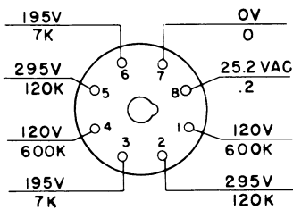
VOLTAGE REGULATOR TUBE V606 6082
