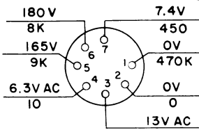
LOCAL A-F OUTPUT TUBE V603 6AK6
