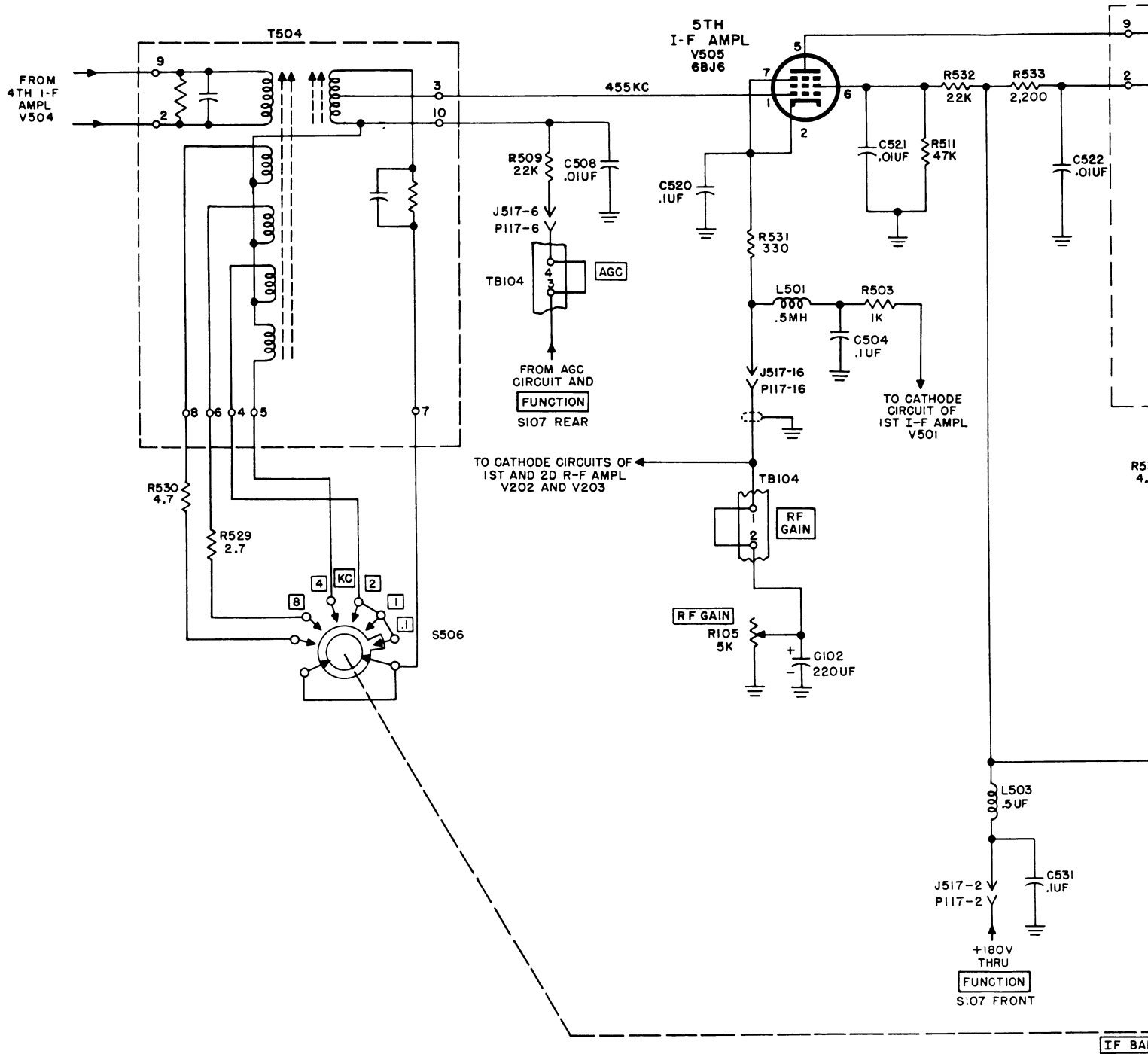
Figure 25. Fifth and sixth if. amplifiers,
