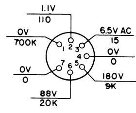
1ST R-F AMPL V202 6BJ6
