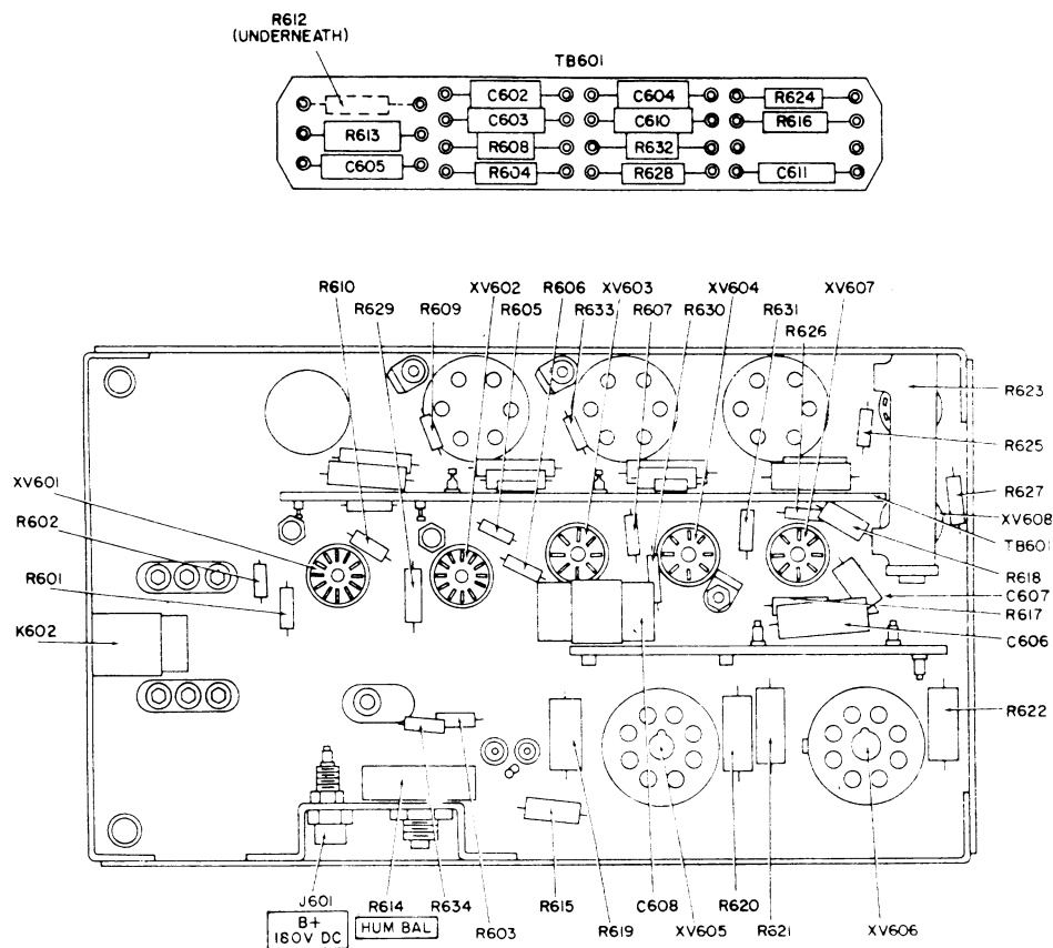
Figure 61. Af subchassis, bottom view.
