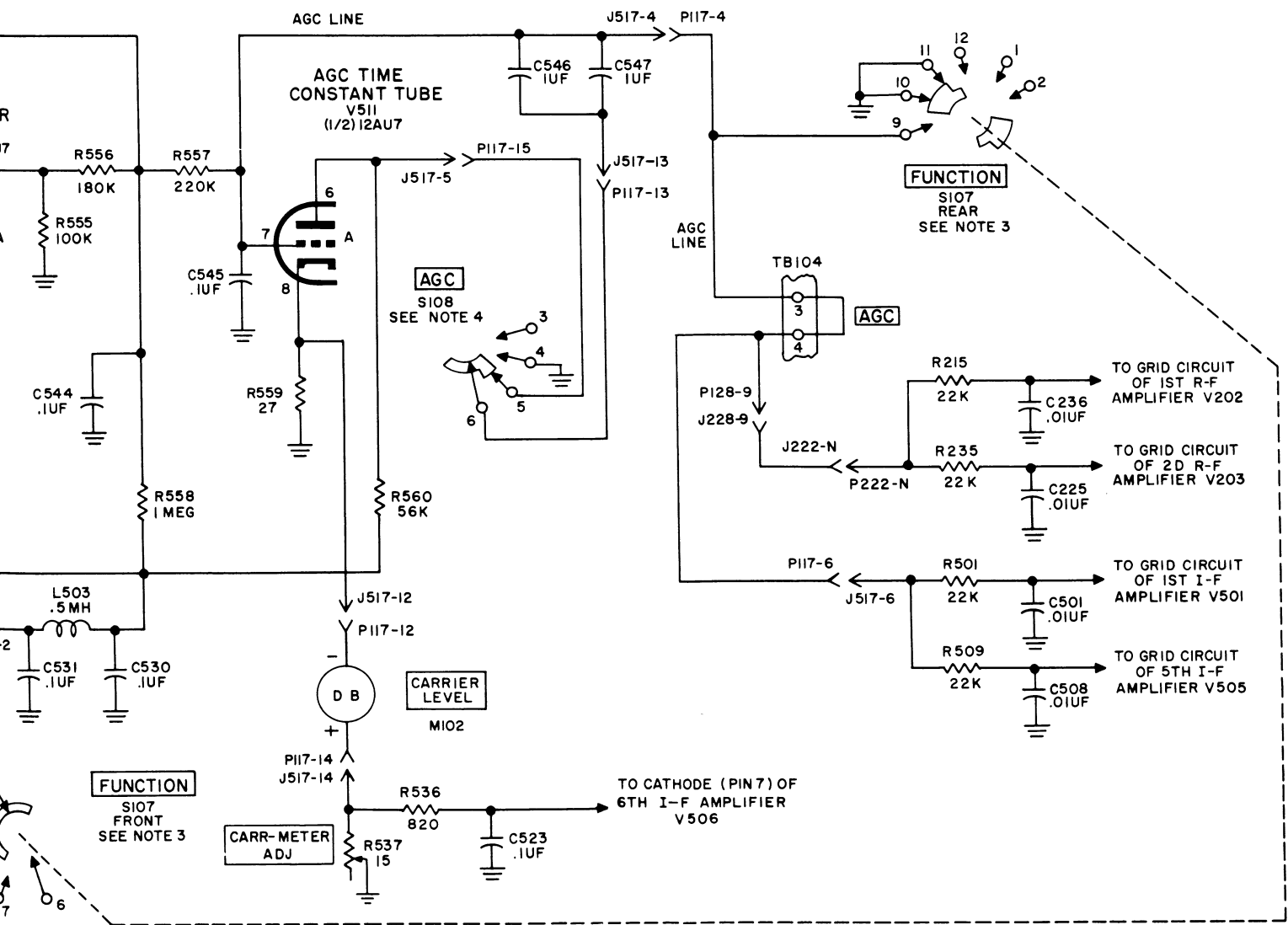
Figure 28. Agc circuit, schematic diagram.
