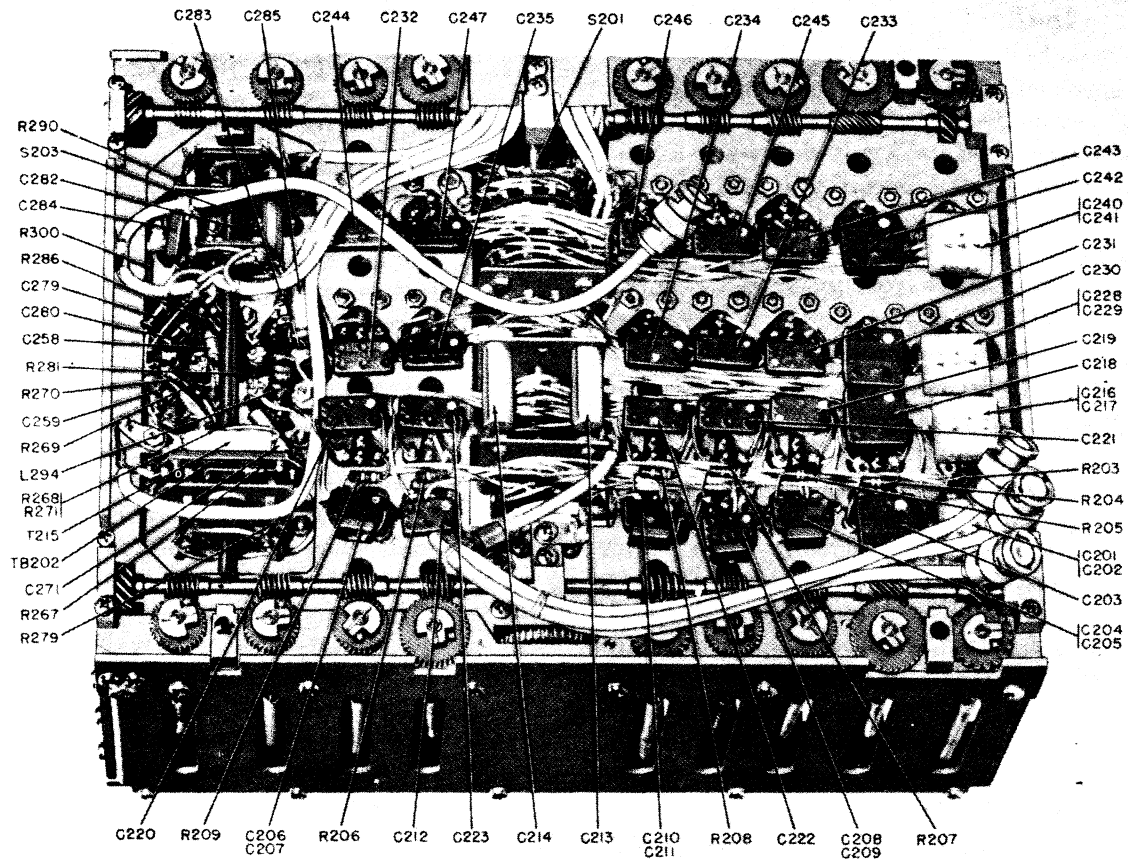
Figure 51. Rf subchassis, bottom view.
