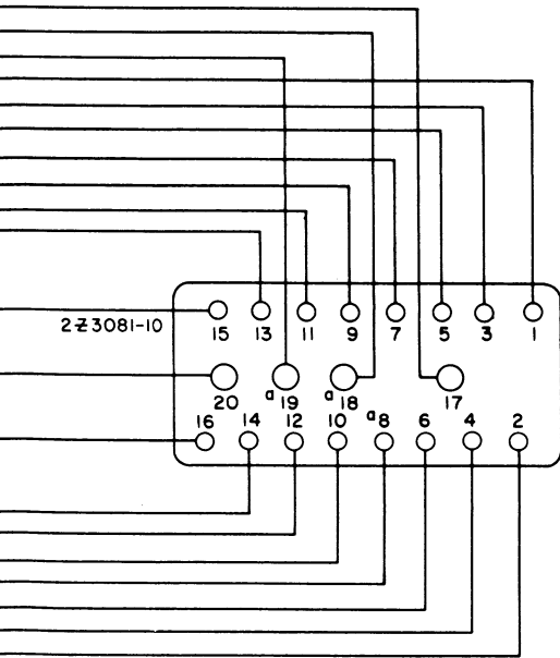
CABLE NO. 2
