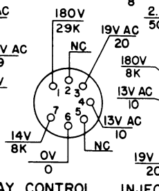
RELAY CONTROL V210 6C4W
