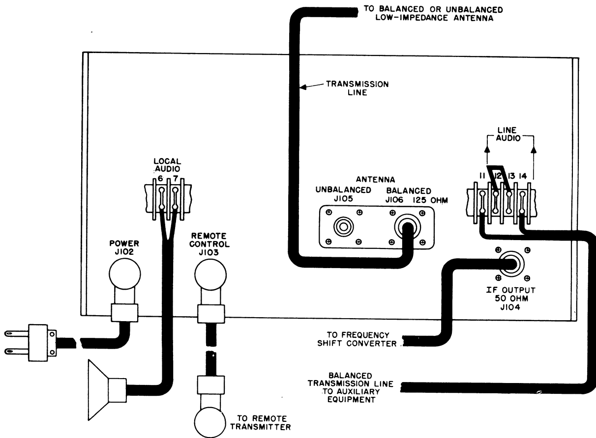
Figure 8. Cording diagram.
