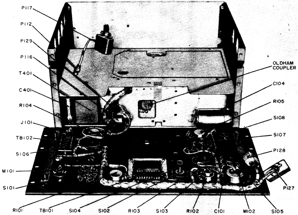
Figure 64. Front panel and main frame, top view.
