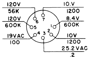
D-C AMPL TUBE V607 6BH6
