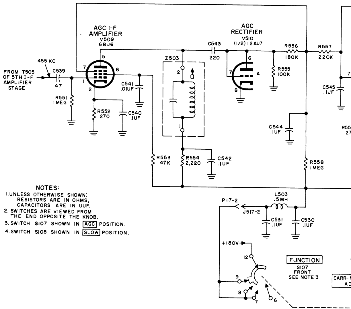
Figure 28. Agc circuit
