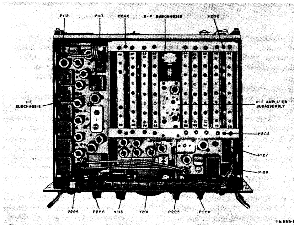
Figure 70. Top view, dust cover and shield removed.
