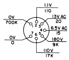
2D R-F AMPL V203 6BJ6
