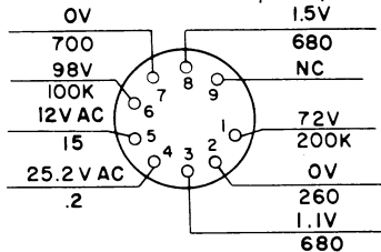
LOCAL A-F AMPL AND LINE A-F AMPL TUBE V602 12AU7
