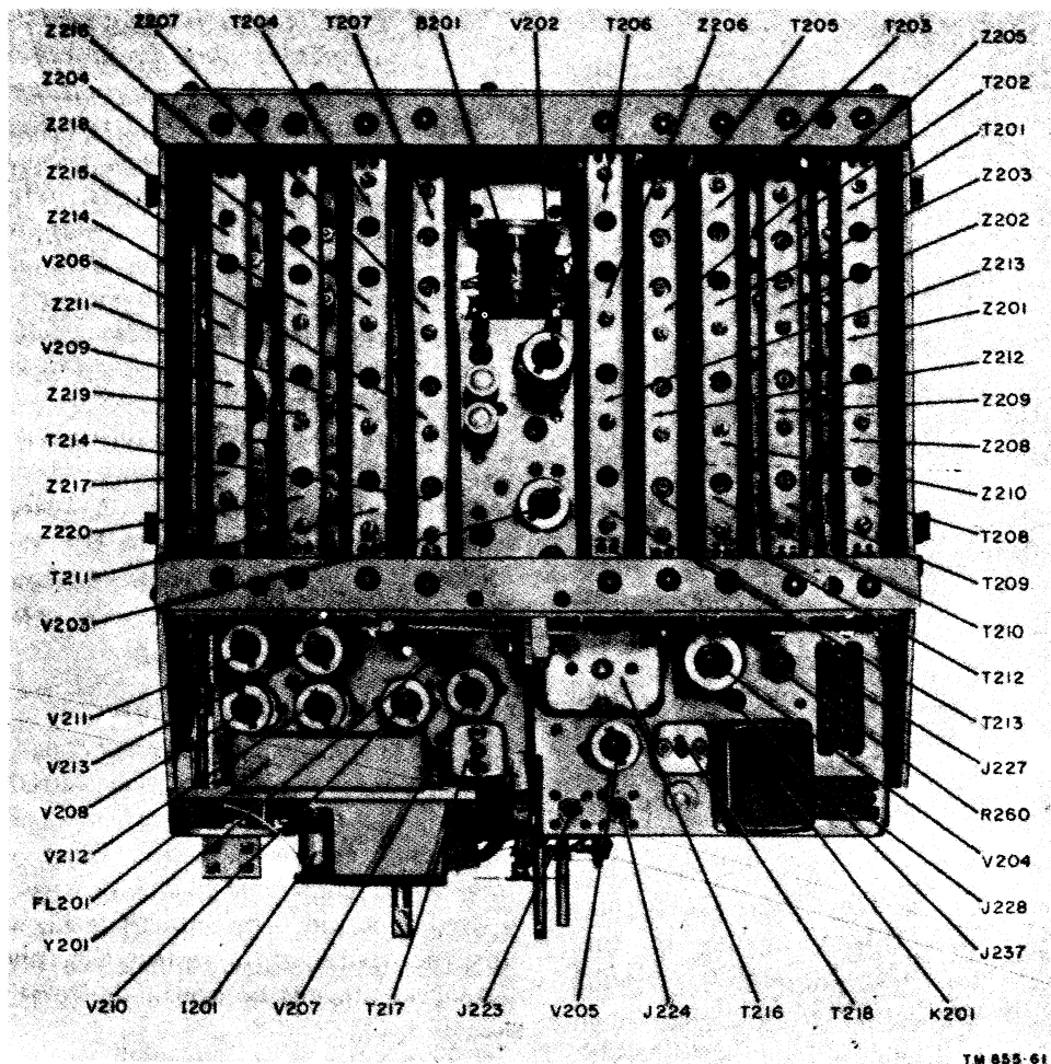
Figure 49. Rf subchassis, top view.
