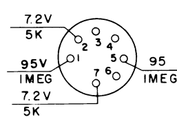
VOLTAGE REFERENCE TUBE V609 5651
