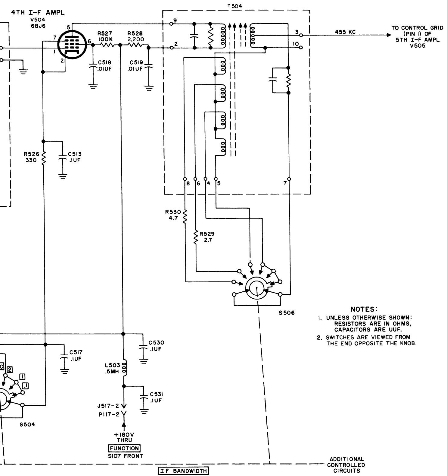
Third and fourth if. amplifiers, schematic diagram.
