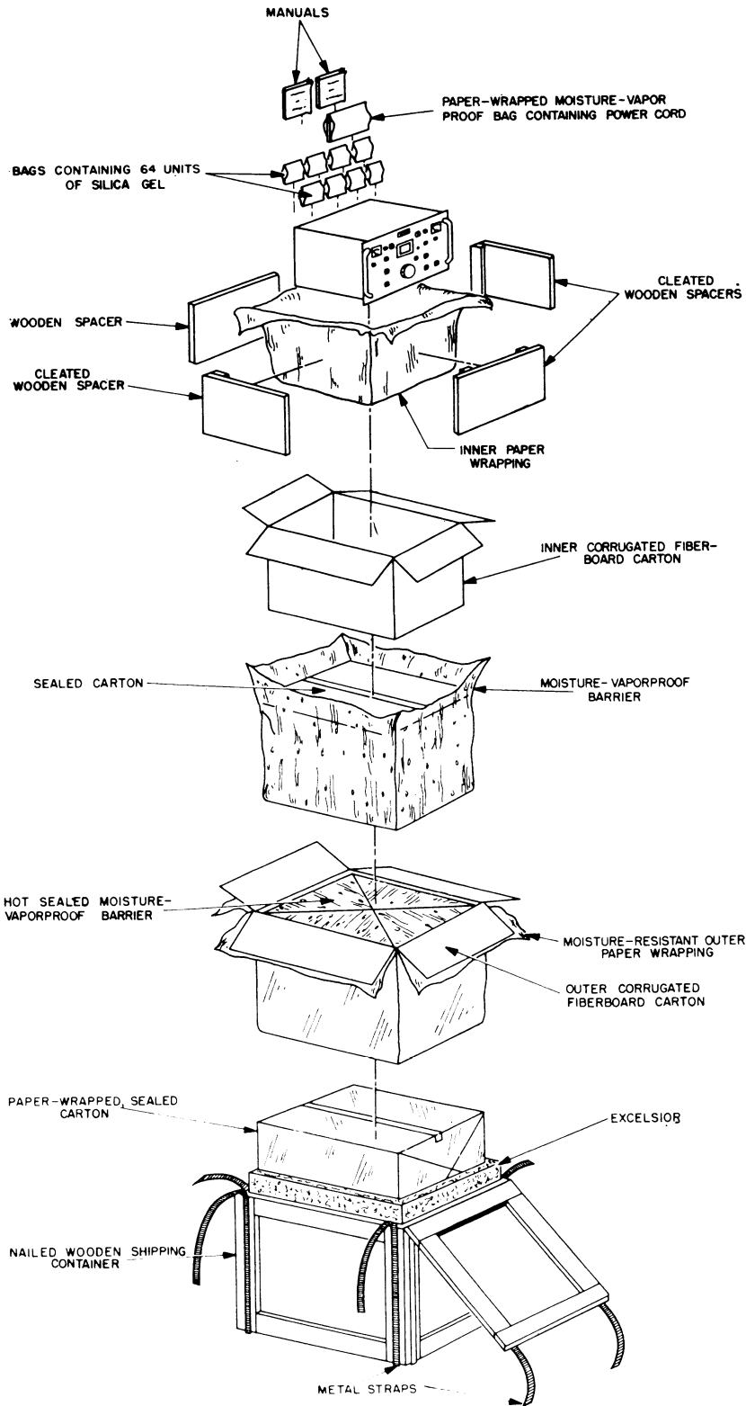
Figure 3. Packaging.
