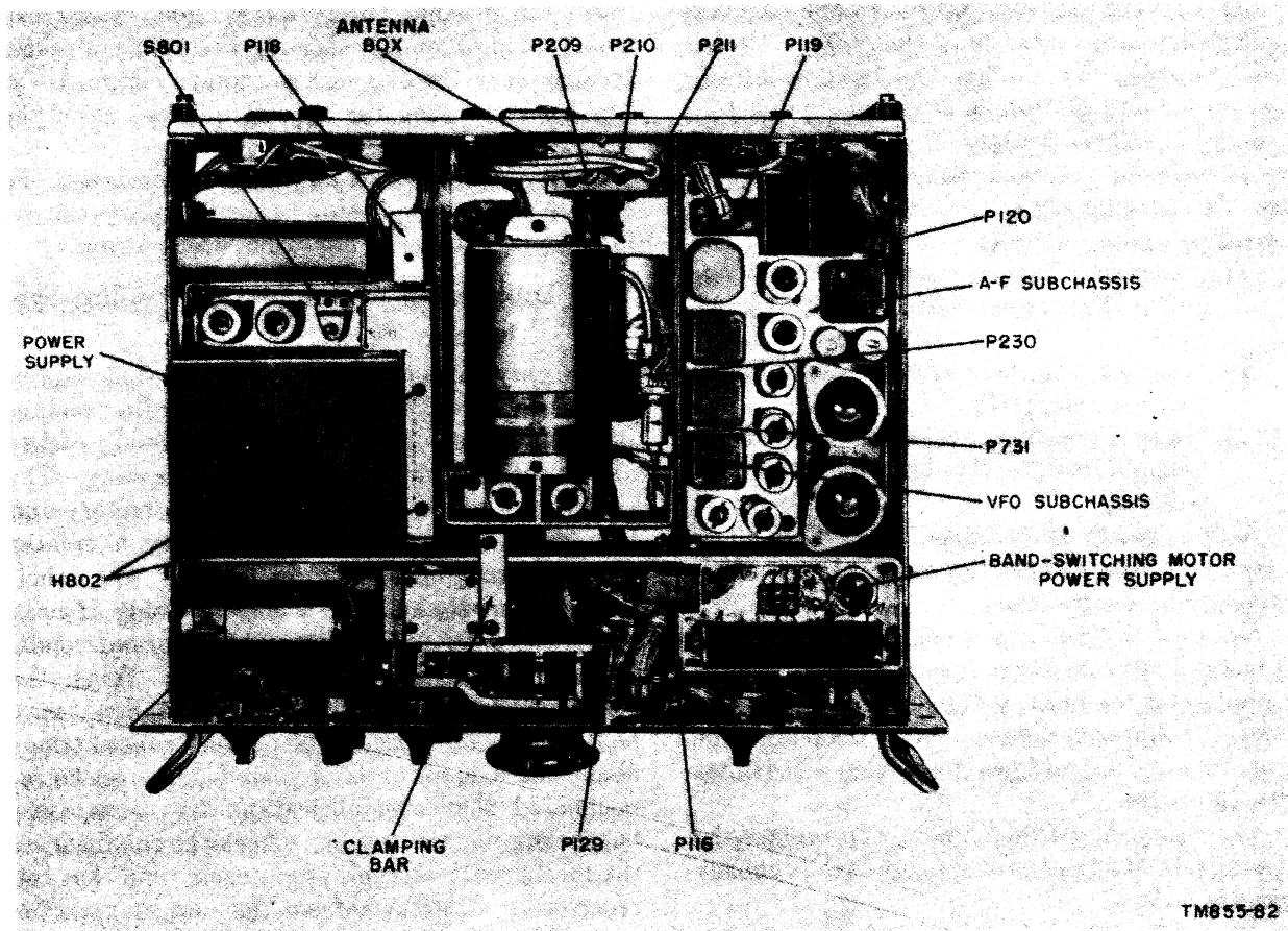
Figure 71. Bottom view, dust cover removed.
