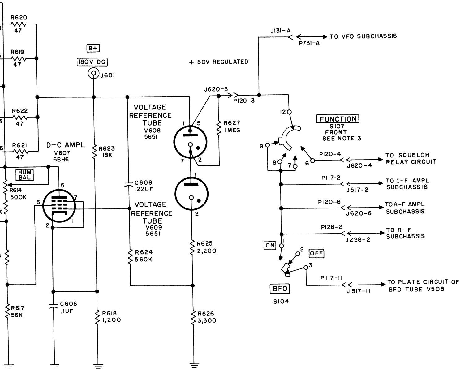
Figure 36. Voltage regulator, schematic diagram.
