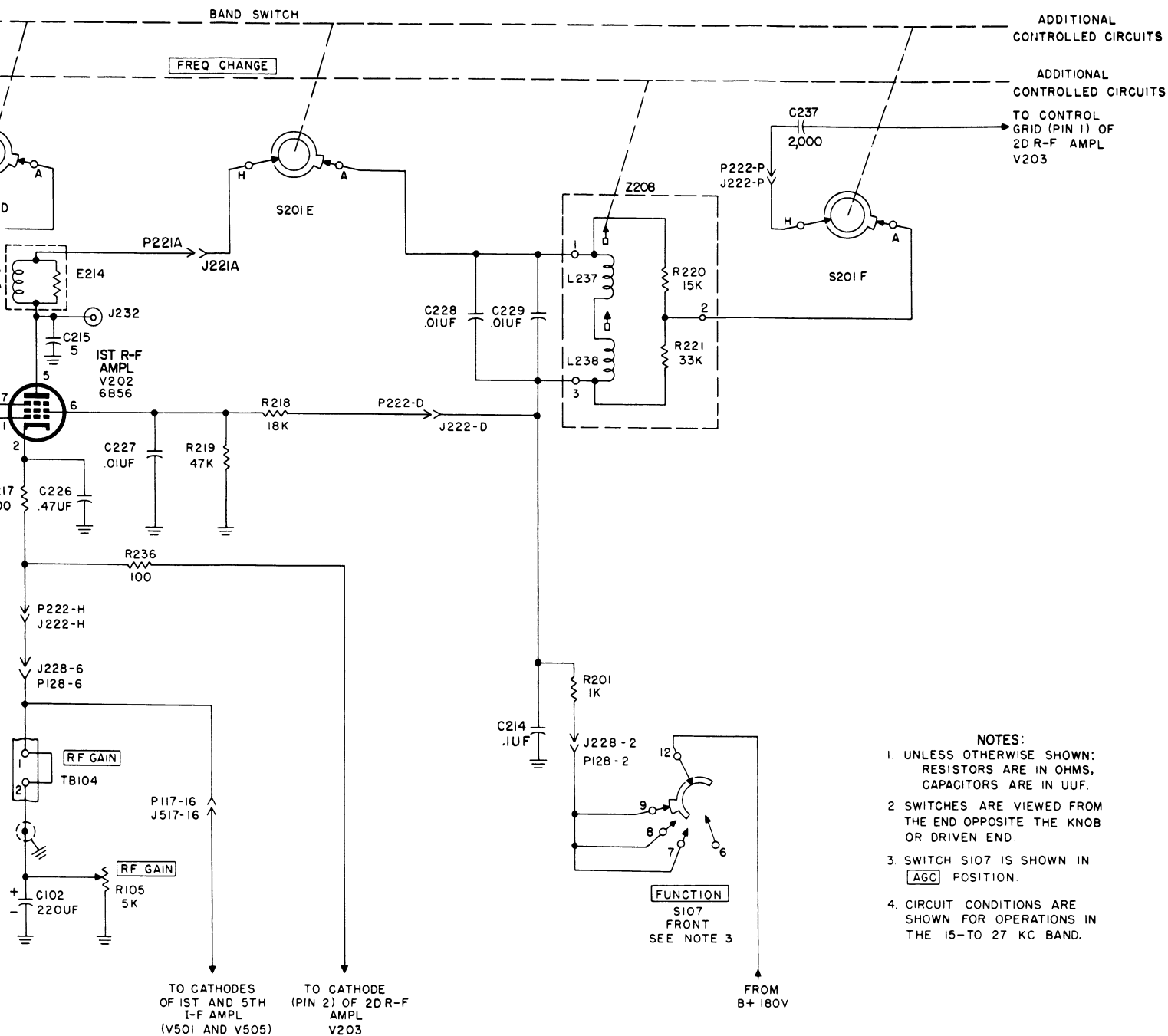
Unit and first rf amplifier, schematic diagram.
