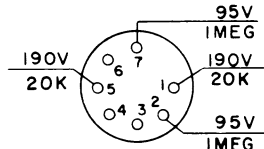
VOLTAGE REFERENCE TUBE V608 5651
