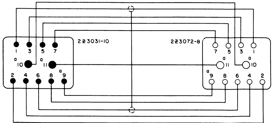
CABLE NO. 3
