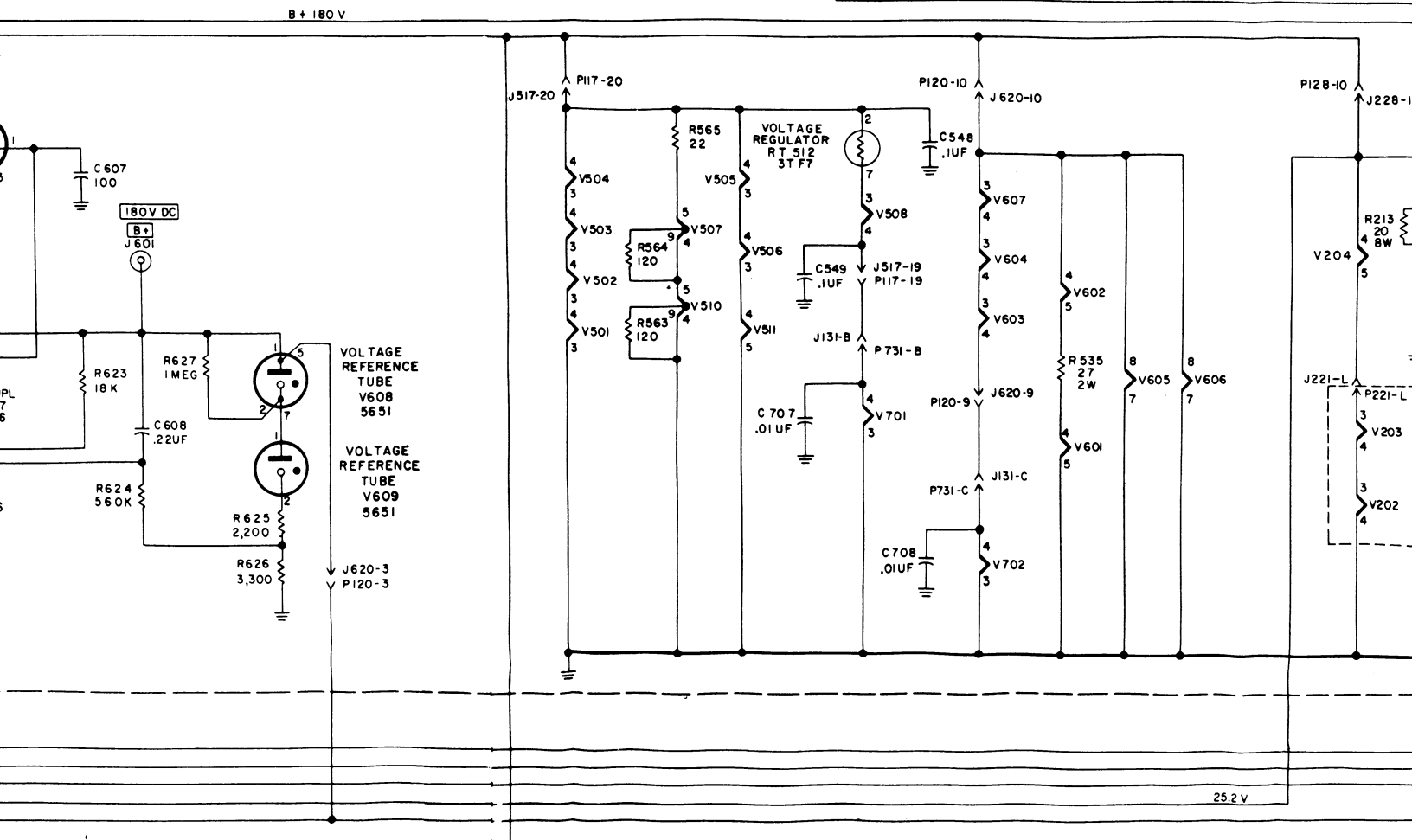
Figure 89. Radio Receiver R-389
