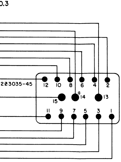
E NO.6 for multiconductor cables.
