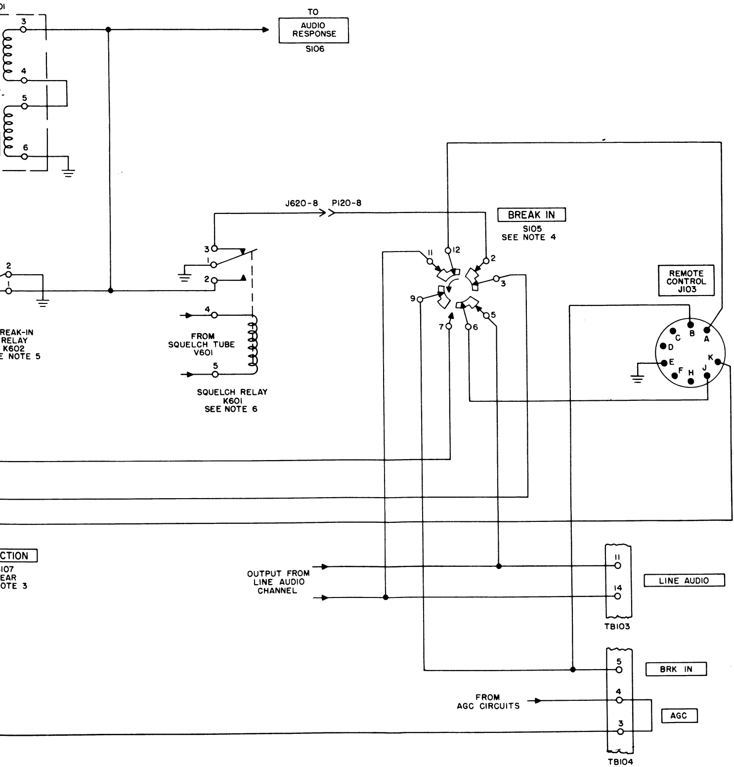
break-in circuit. schematic diagram.
