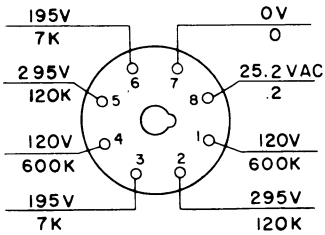
VOLTAGE REGULATOR TUBE V605 6082
