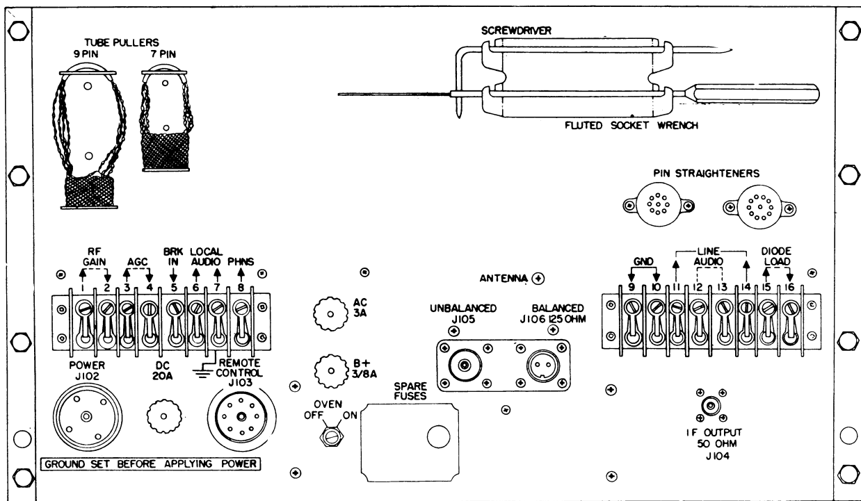
Figure 7. Back panel.
