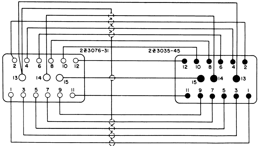
CABLE NO. 5
