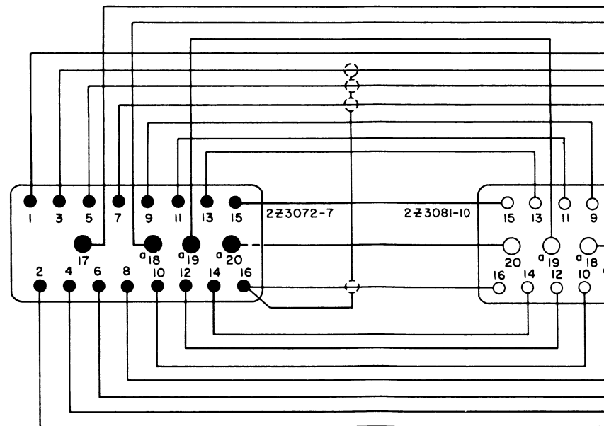
CABLE NO. 2
