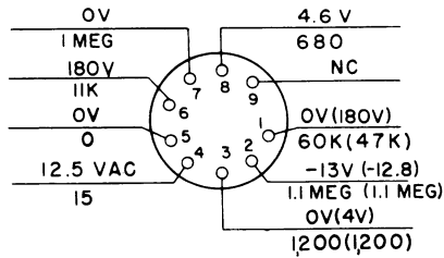
A-F AMPL AND SQUELCH TUBE V601 12AU7
